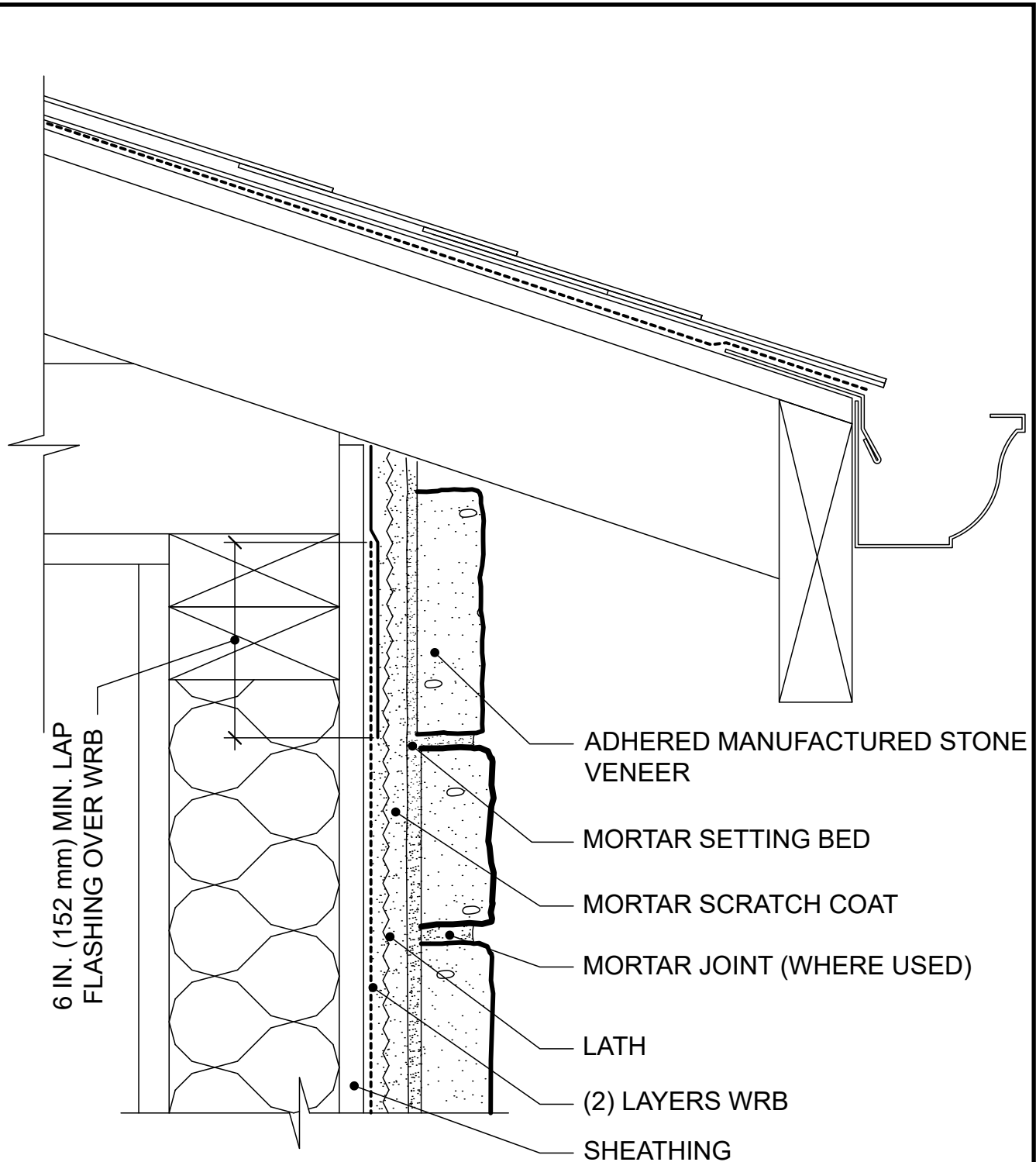
Figure 13a. Open Eave - Overhang
