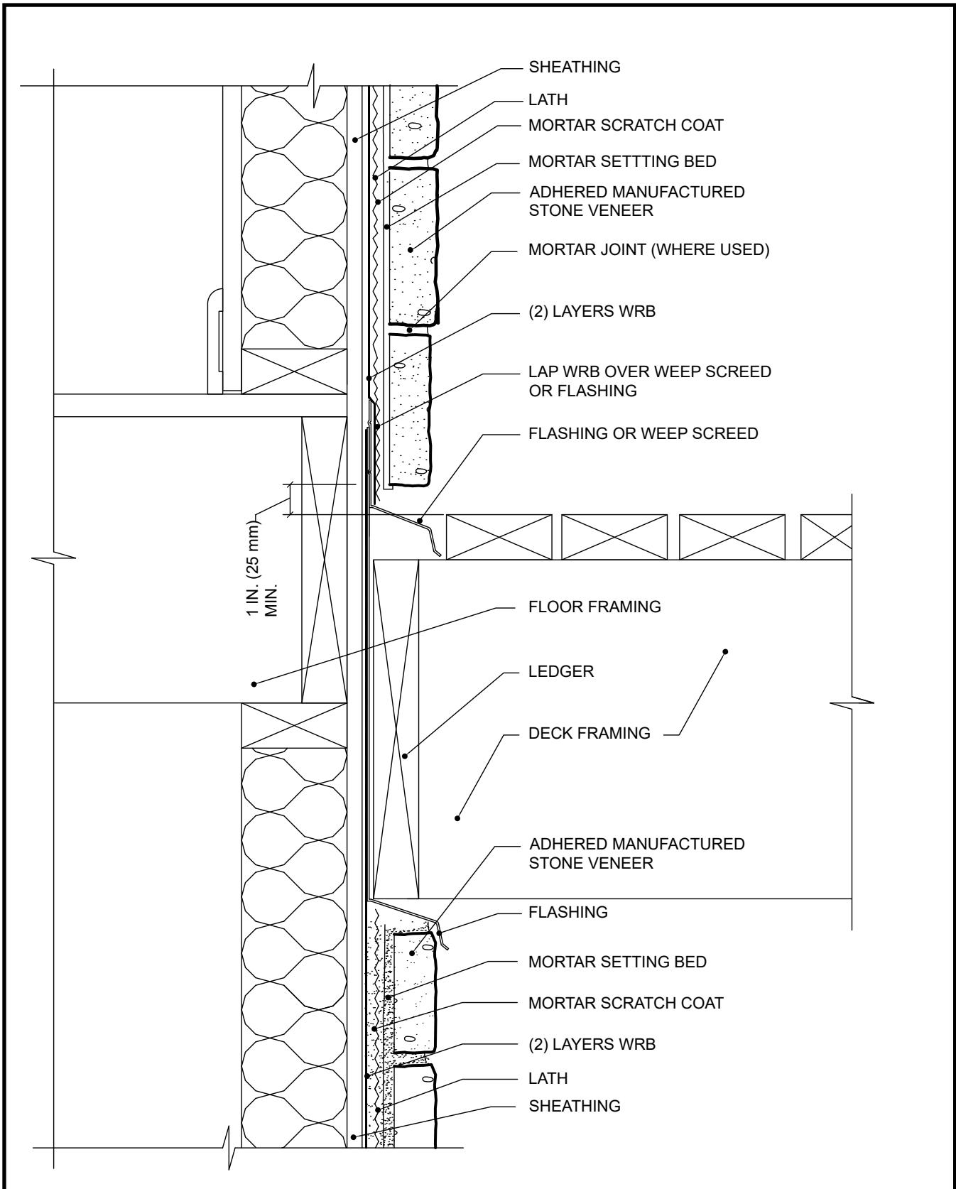
Figure 33. Deck Termination
