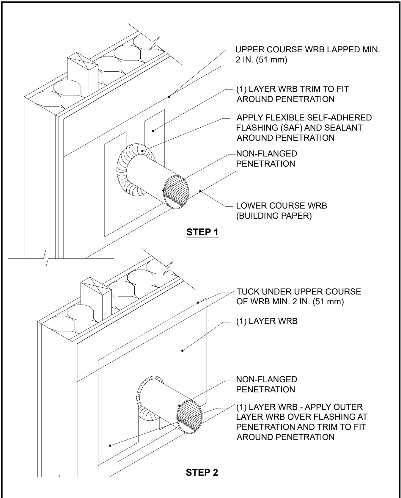
Figure 29. Penetration Non-Flanged, with Building Paper WRB
