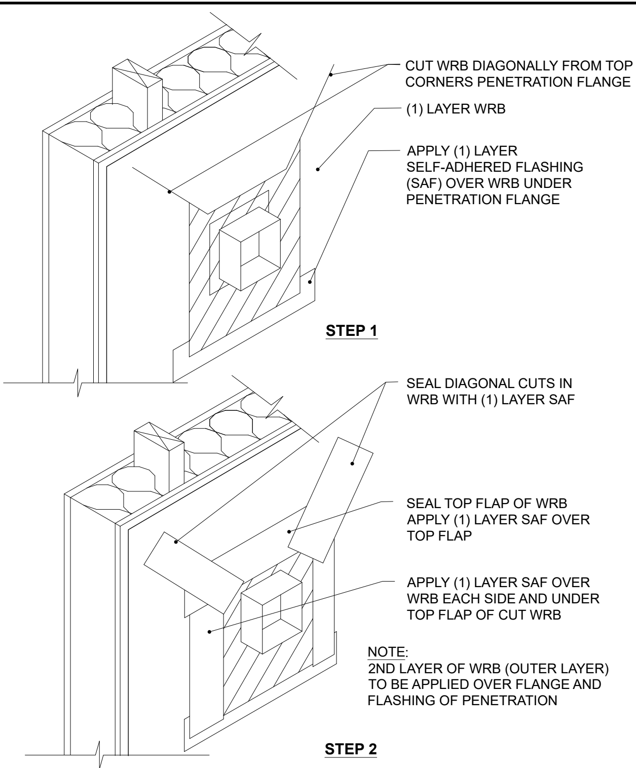
Figure 28. Penetration, Flanged
