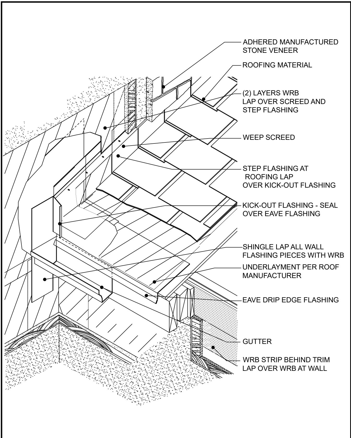
Figure 24. Kick-Out Flashing
