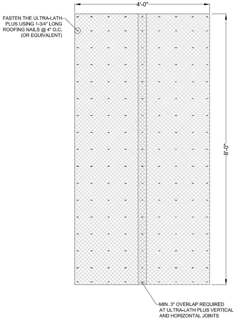
FIGURE 1 - Assembly (Continued)
